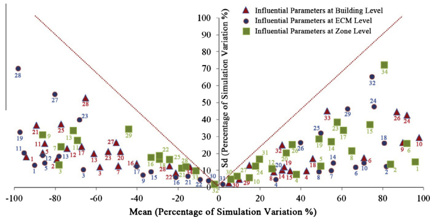
Fig. 6. Mean and standard deviation of the elementary effects on the energy simulation for the influential parameters at the building level, ECM level and zone level.
