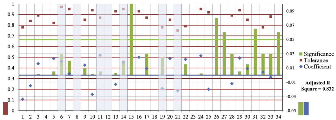
Fig. 7. Multi-regression analysis results at the building level ( F = 57.24 ) – See Table 2a for parameter IDs (Estimable parameters and ECM control related parameters are shaded).
