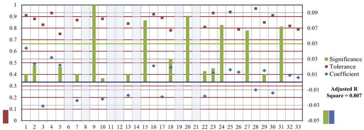
Fig. 9. Multi-regression analysis results at the zone level ( F = 41.59 ) – See Table 2c for parameter IDs (Estimable parameters and ECM control related parameters are shaded).
